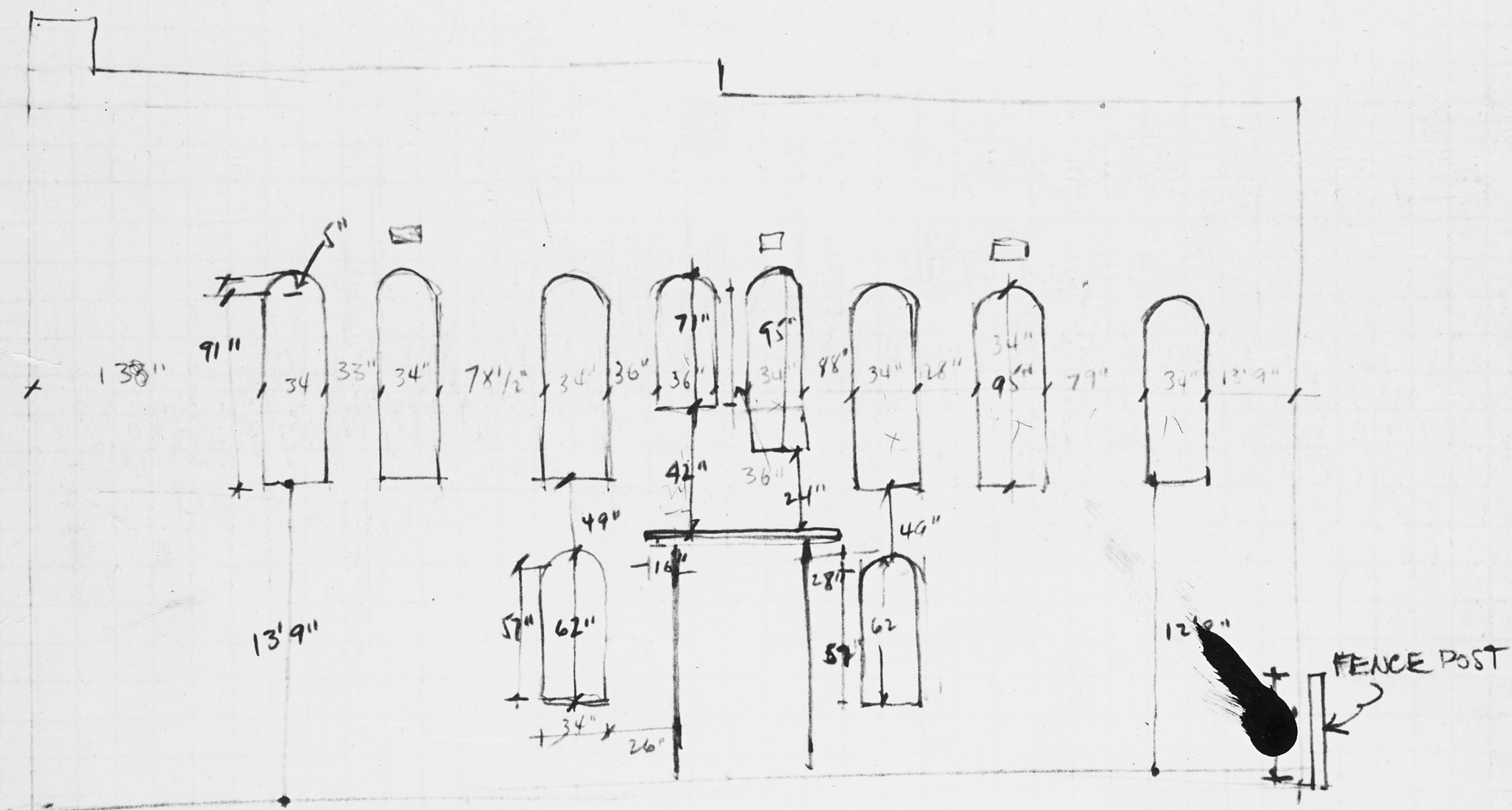
95 71 24 ELEVATION BUILDING "A" LOOKING NORTH
